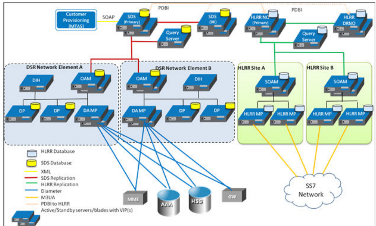
Figure 8-2 SDS/HLRR Architecture Overview
